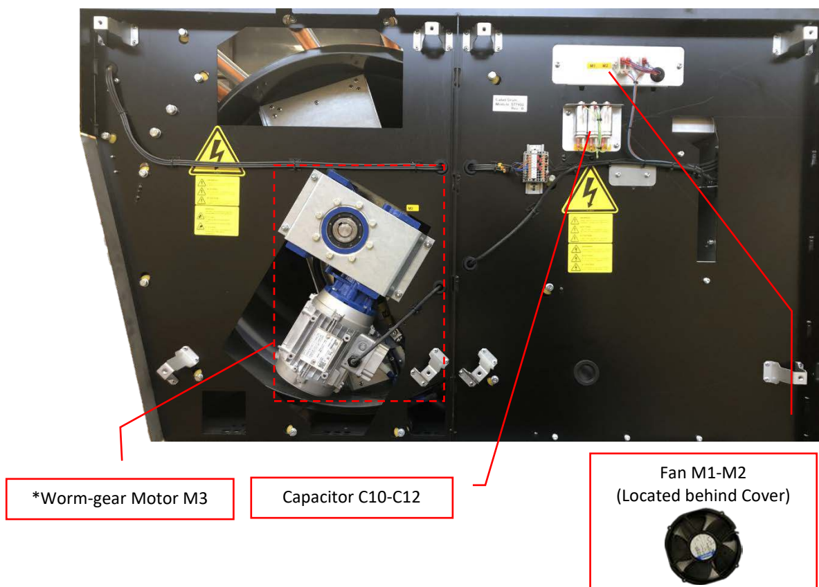
Figure 5: Right Side Internal Components
