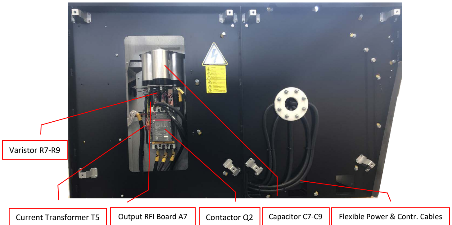
Figure 4: Left Side Internal Components
