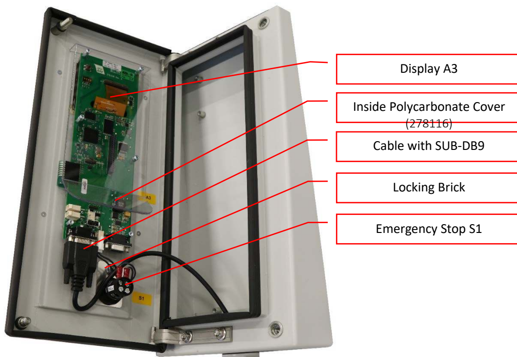
Figure 9: Remote Control Box Internal View
