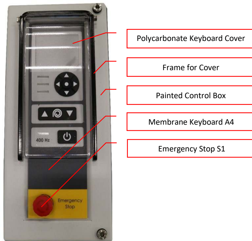
Figure 8: Remote Control Box Front View
