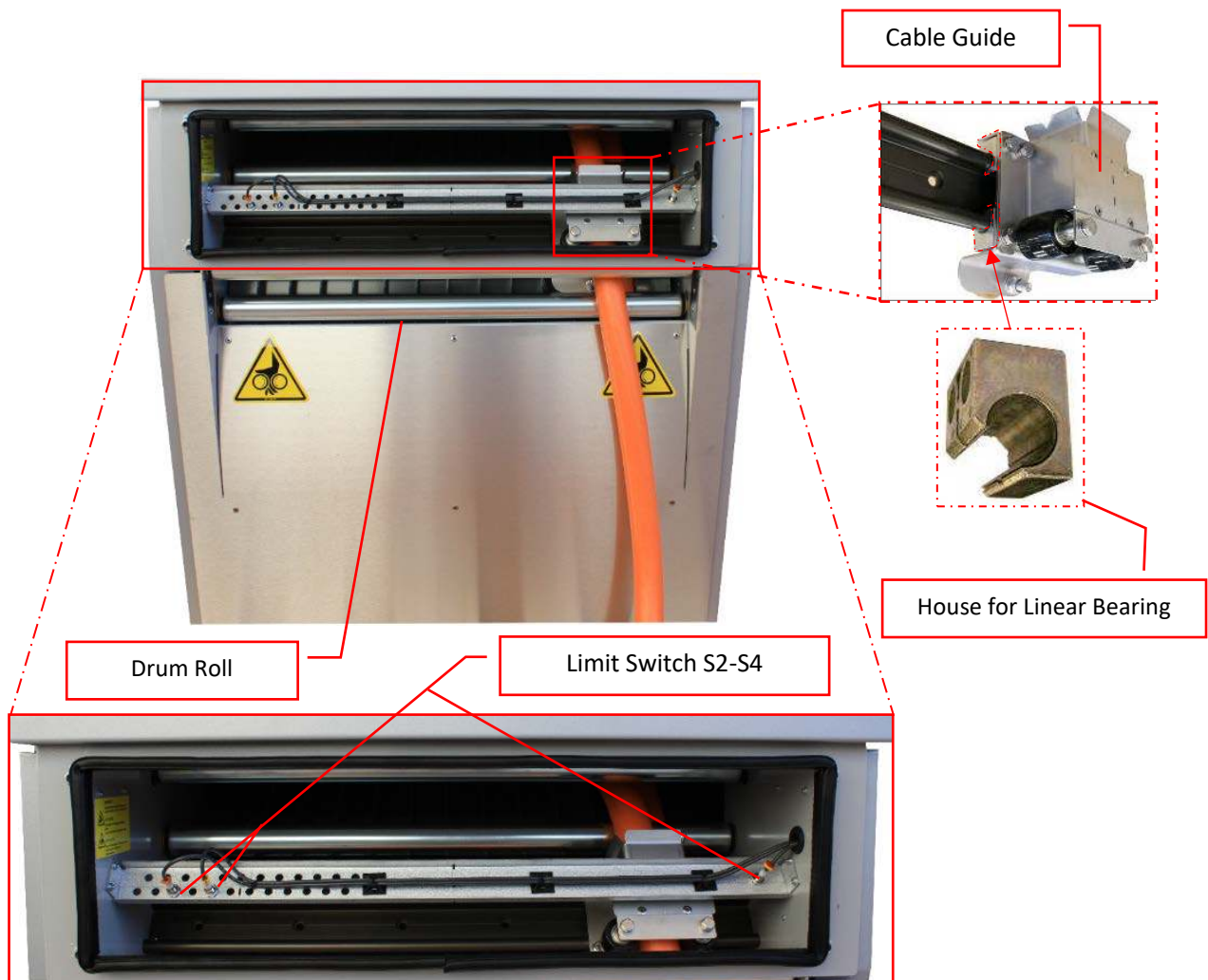
Figure 7: Output Side Cable Guide
