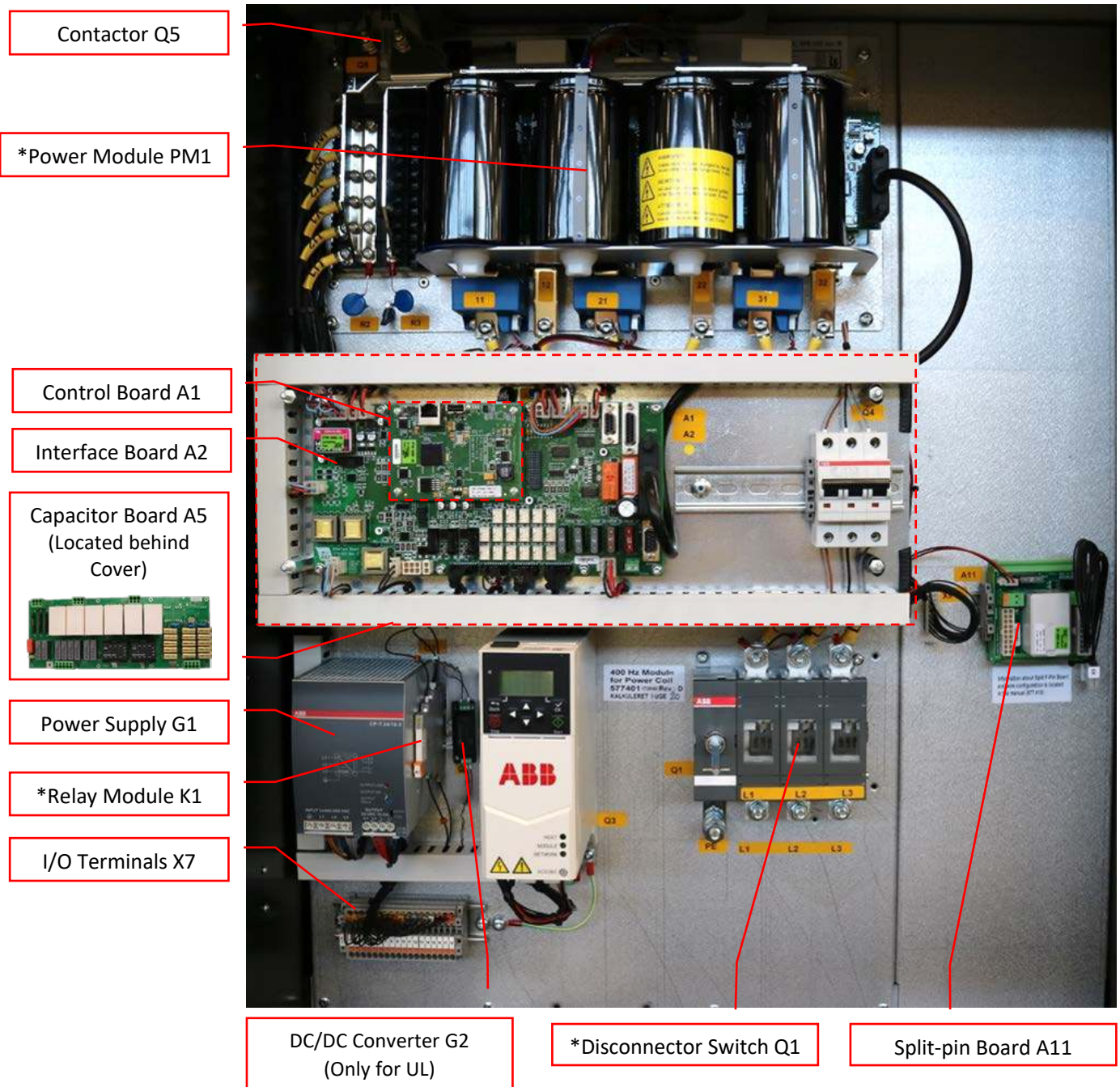
Figure 3: Input Side Internal Components
