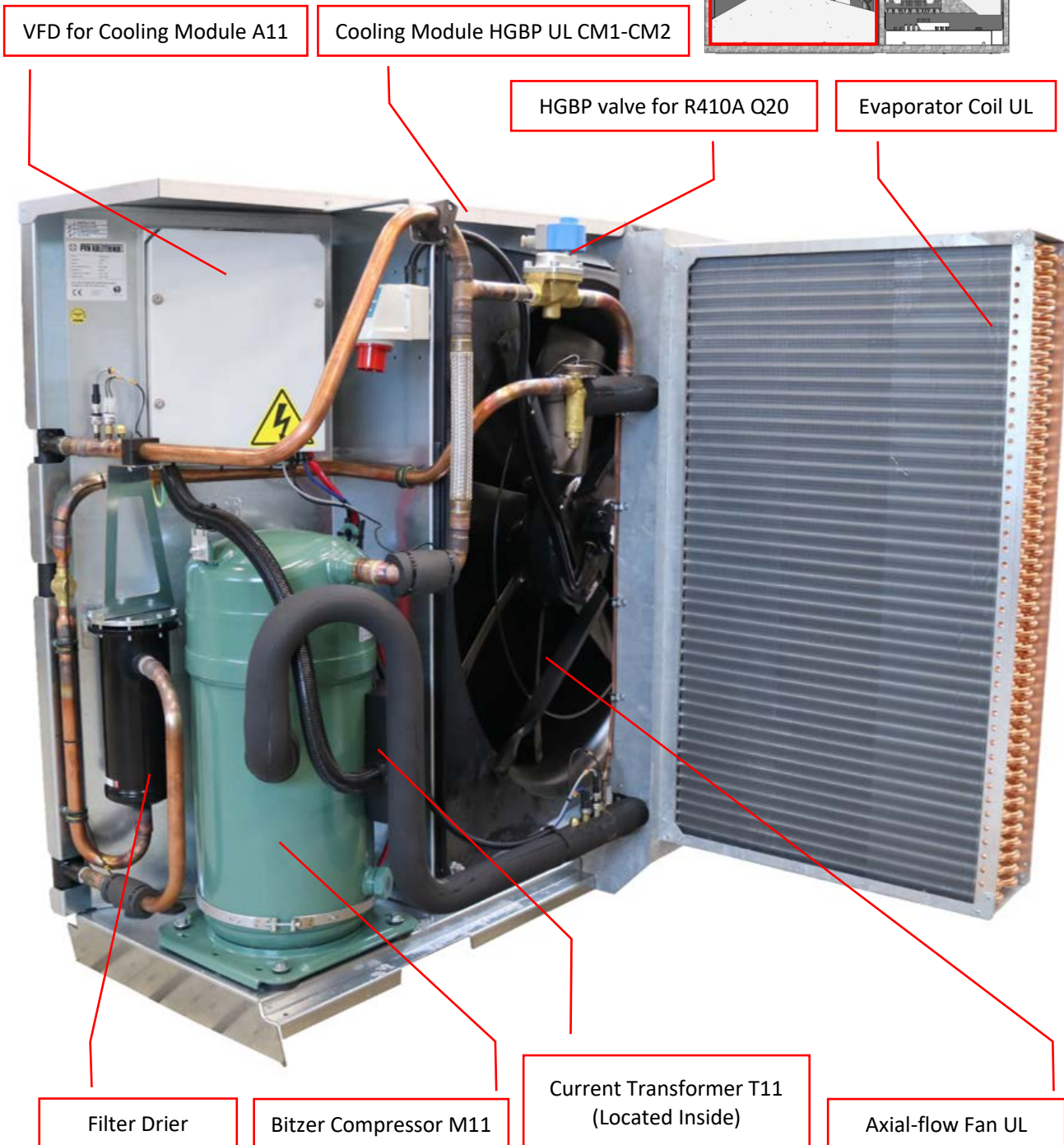
Figure 8: Cooling Module 1 of 2
