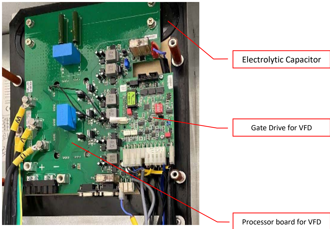
Figure 12: VFD Inside
