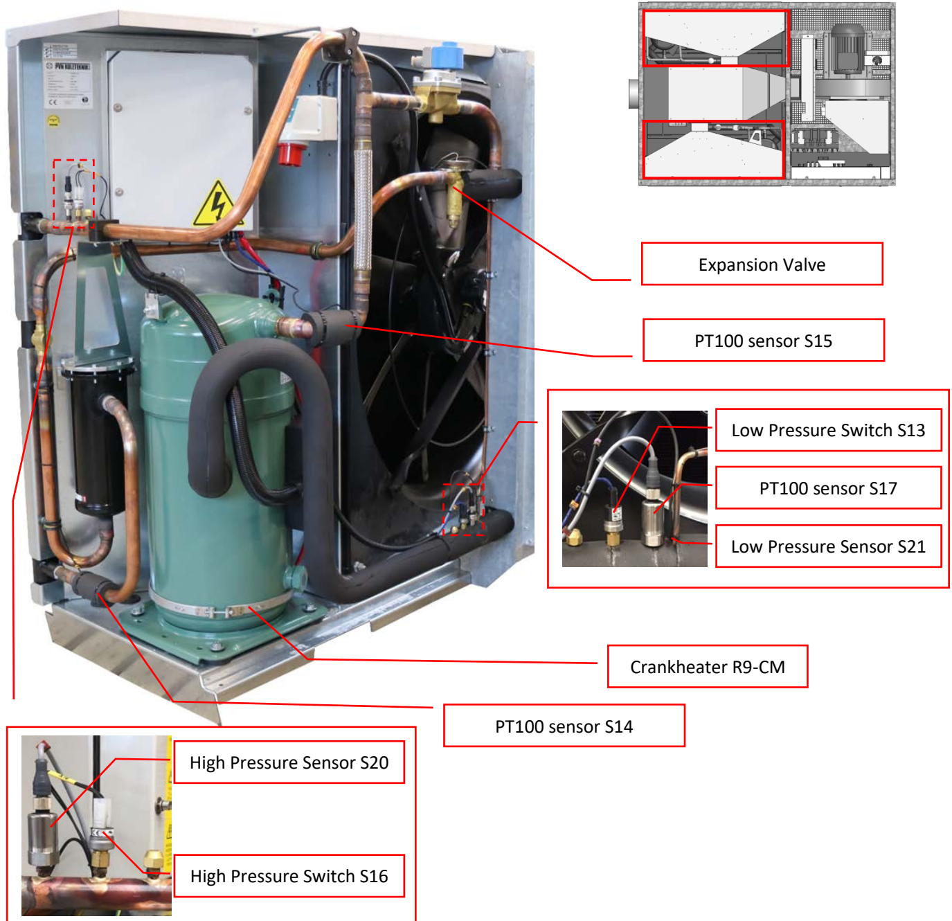
Figure 9: Cooling Module 2 of 2
