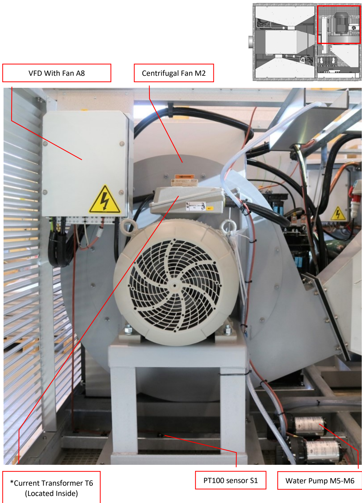
Figure 5: Main Blower zone
