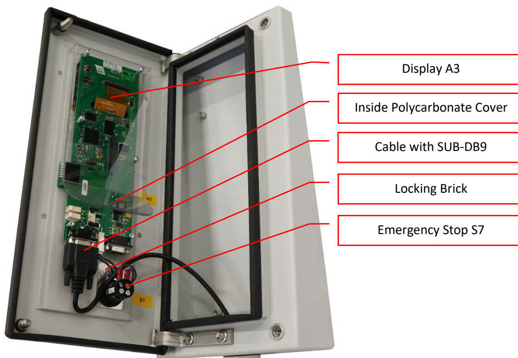
Figure 11: Remote Control Box Internal
