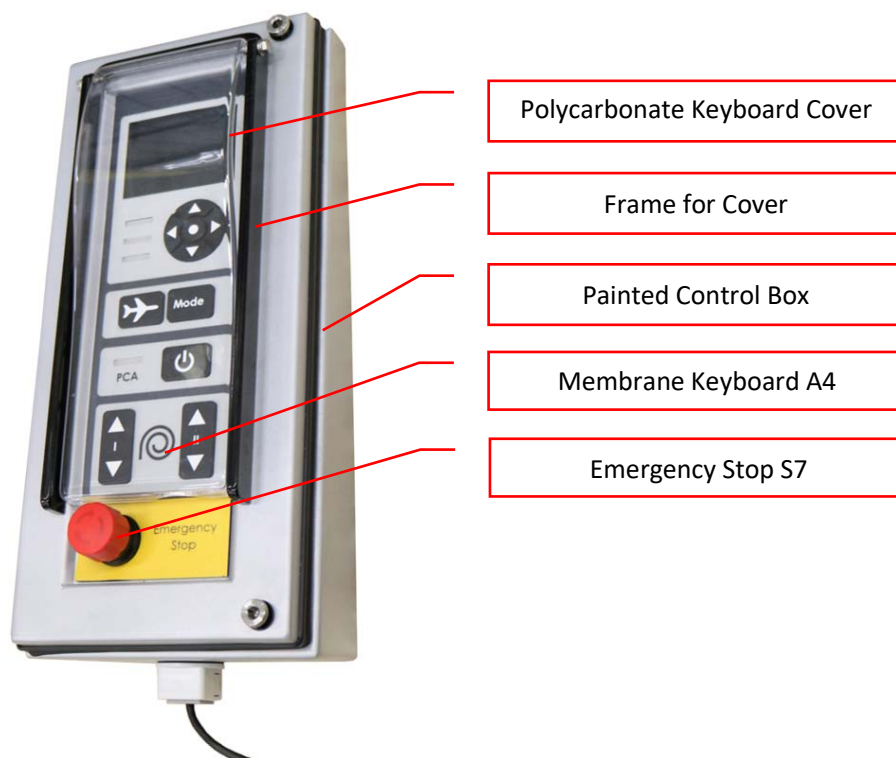
Figure 10: Remote Control Box Front
