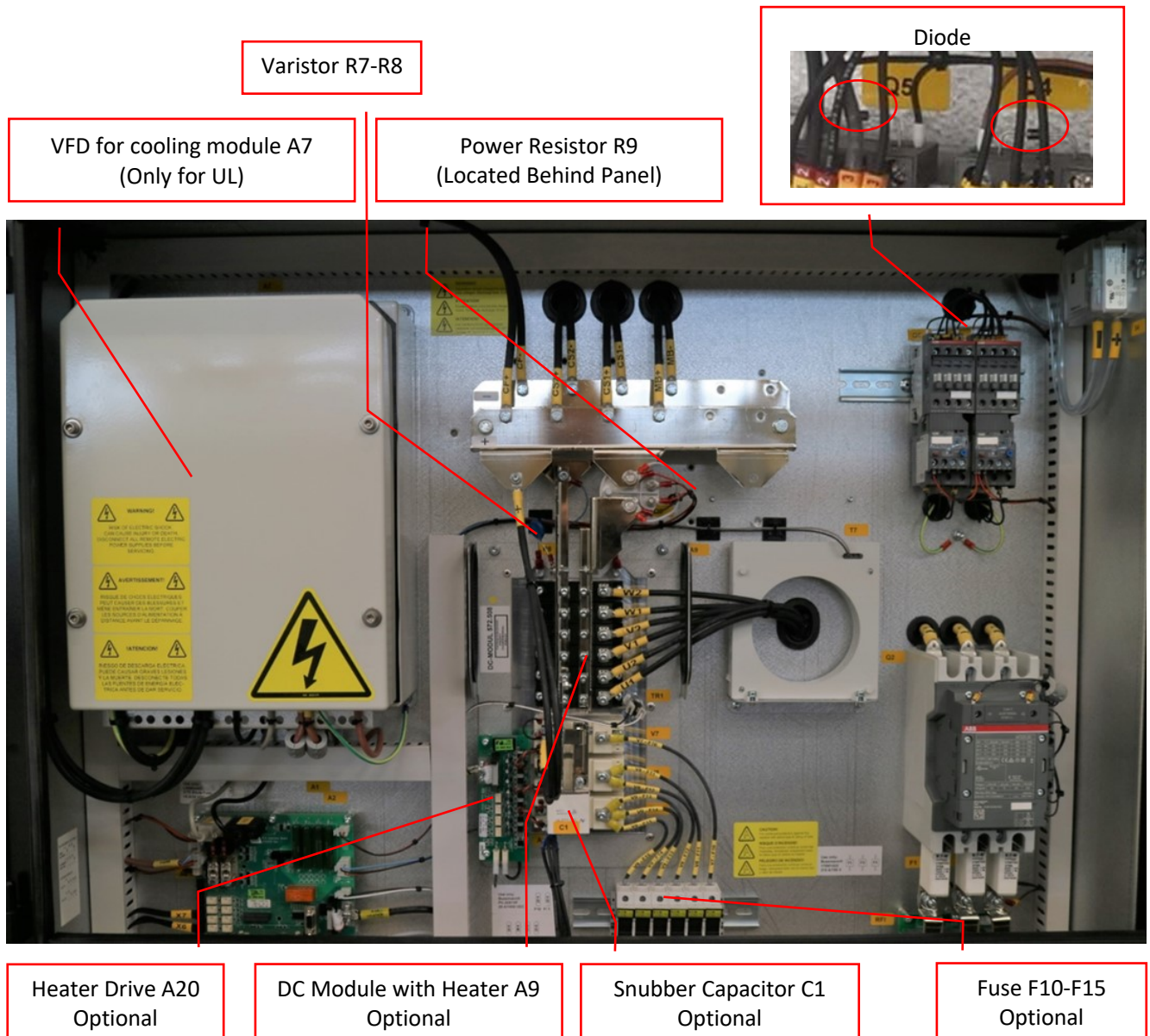
Figure 3: Electronic zone High 2 of 2
