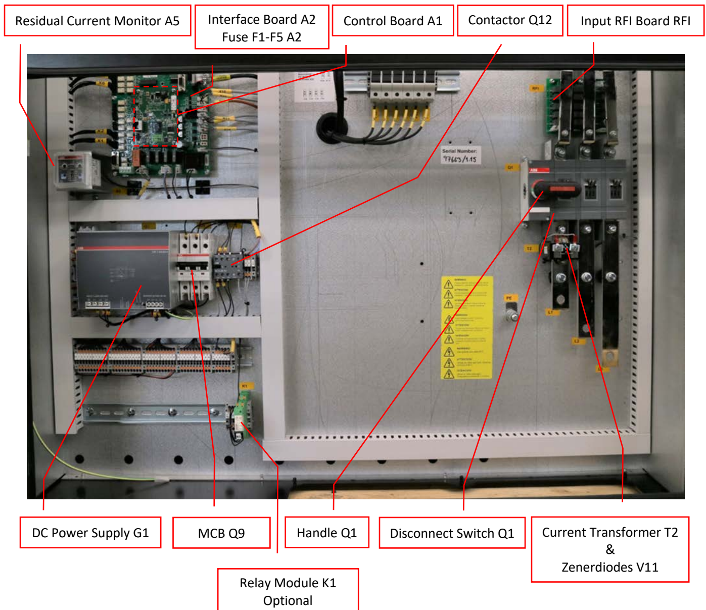
Figure 4: Electronic zone Low
