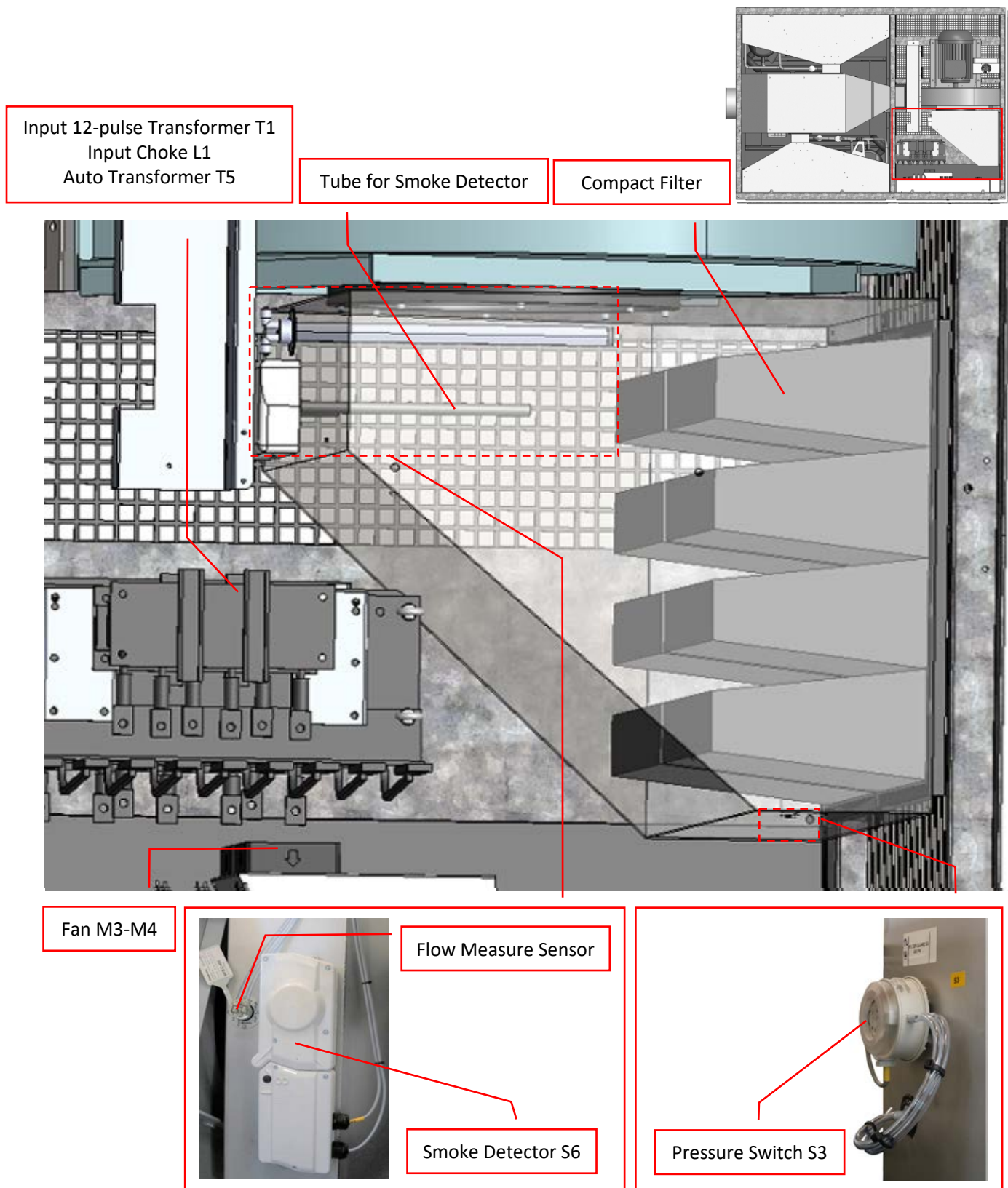
Figure 6: Air Inlet & Internal Electrical zone
