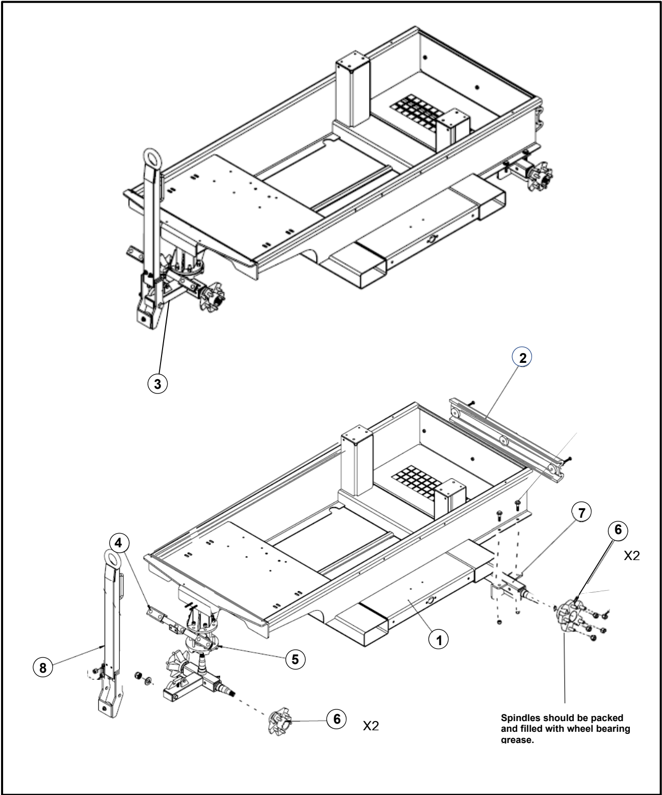
Figure 3-2, 4400-T3/JetEx8 Assy, Chassis/Running Gear (Sheet 1 of 2).
