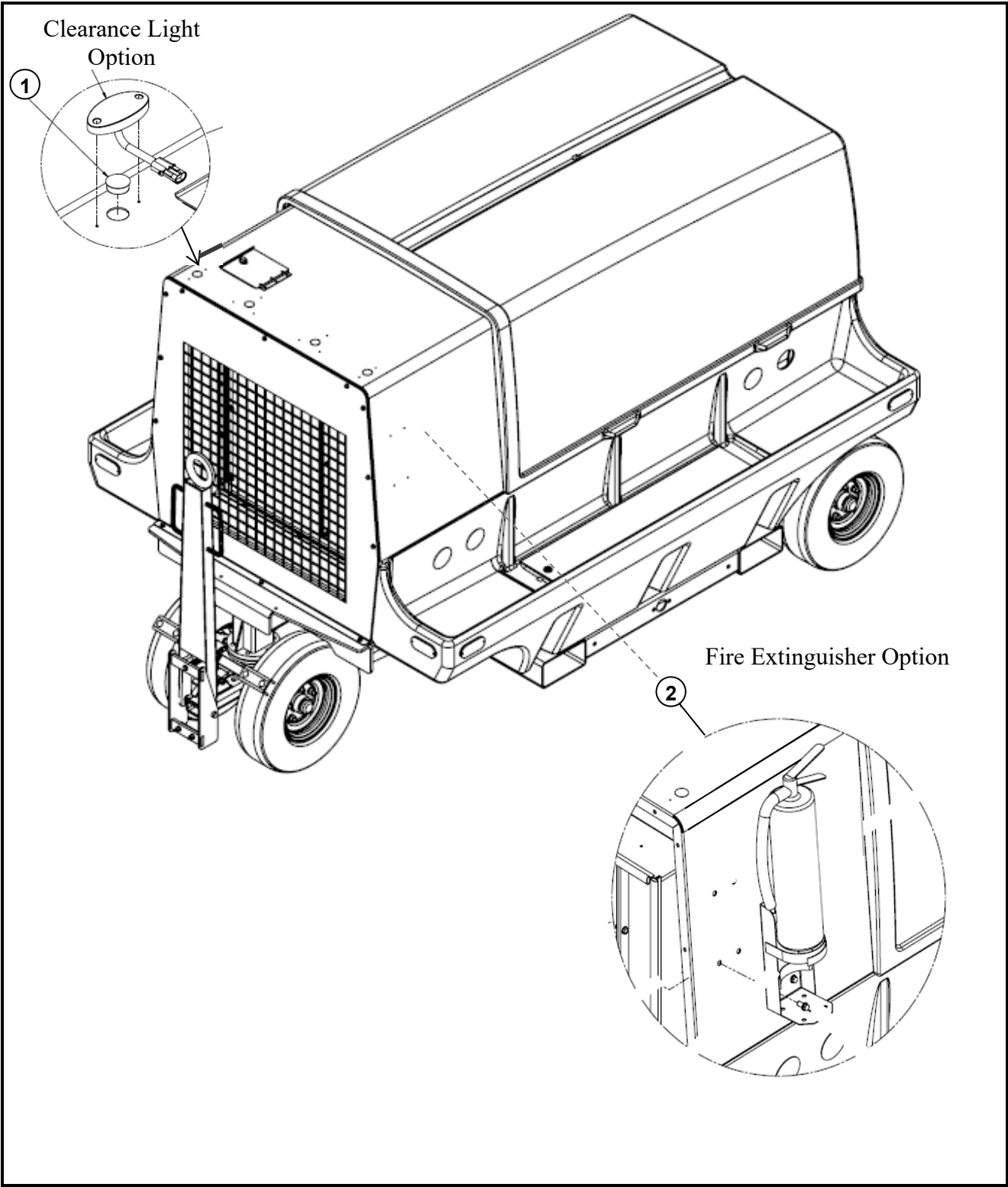
Figure 3-1. 4400-T3, 60/90/100 kVA, 3-Phase 115 Volt Generator Set (Sheet 1 of 3).
