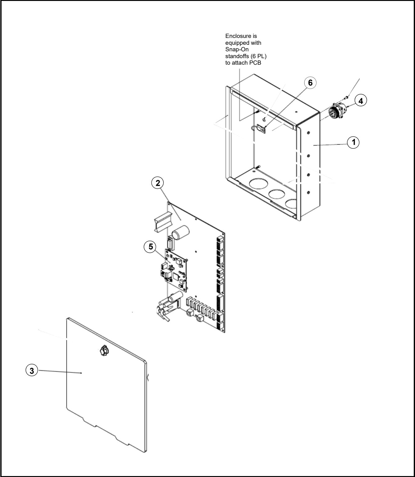
Figure 3-10. 4400-T3, Control Module Box Assembly 60/90/100 kVA (Sheet 1 of 2).
