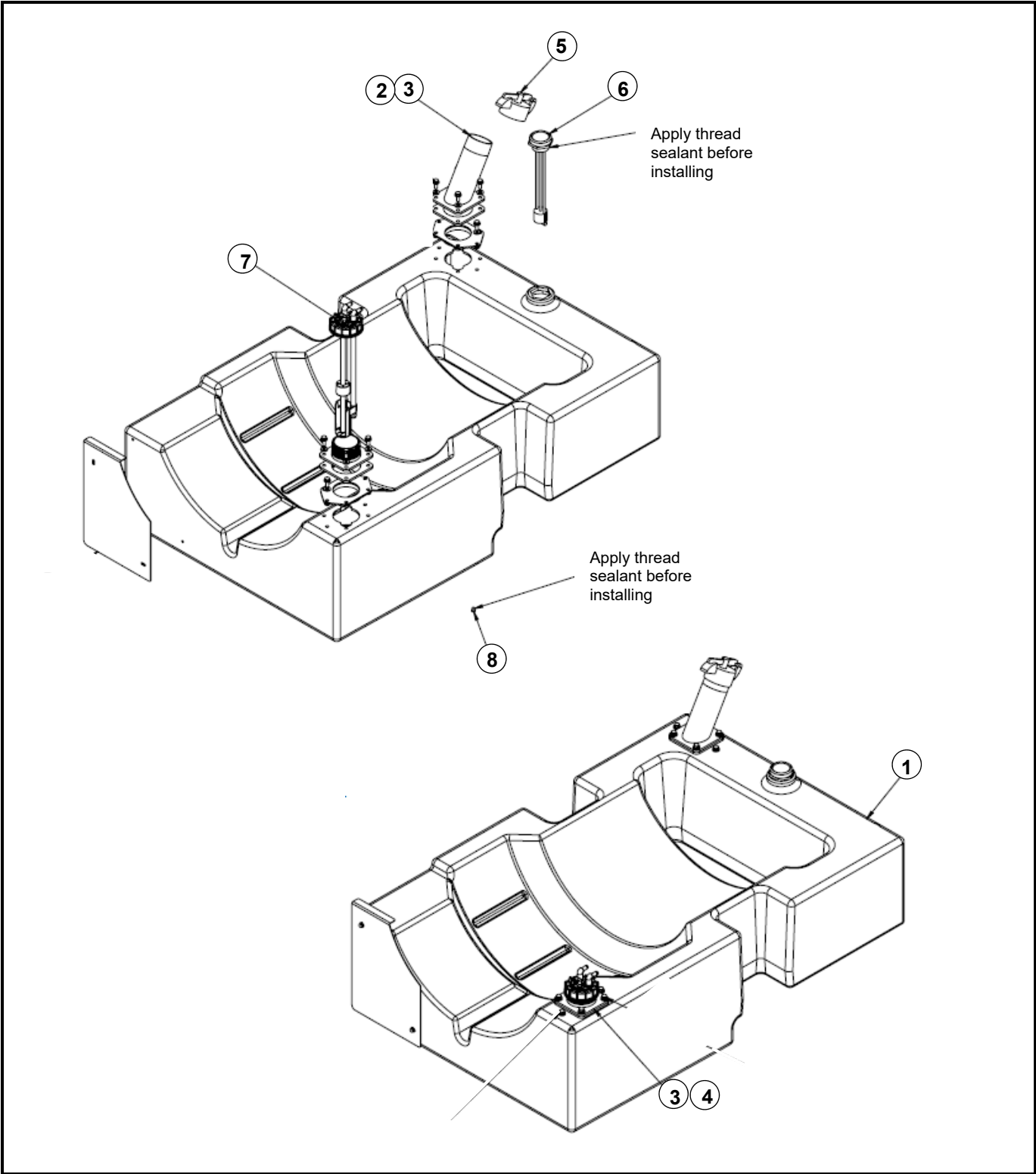
Figure 3-5. 4400-CP, Fuel Tank Composite Assembly, Common Platform (Sheet 1 of 2).
