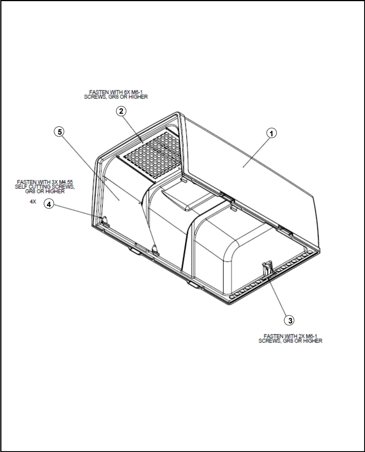
Figure 3-11. 4400-CP, Cable Tray Assembly, Left Side 60/90/100 kVA (Sheet 2 of 2).
