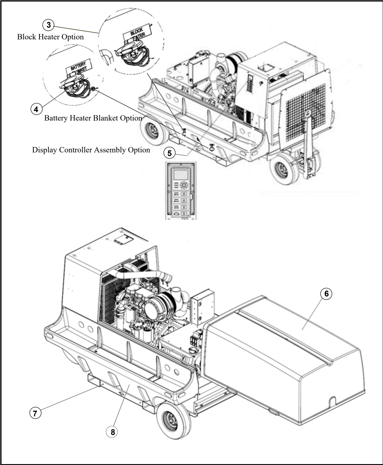
Figure 3-1. 4400-T3, 60/90/100 kVA, 3-Phase 115 Volt Generator Set (Sheet 2 of 3).
