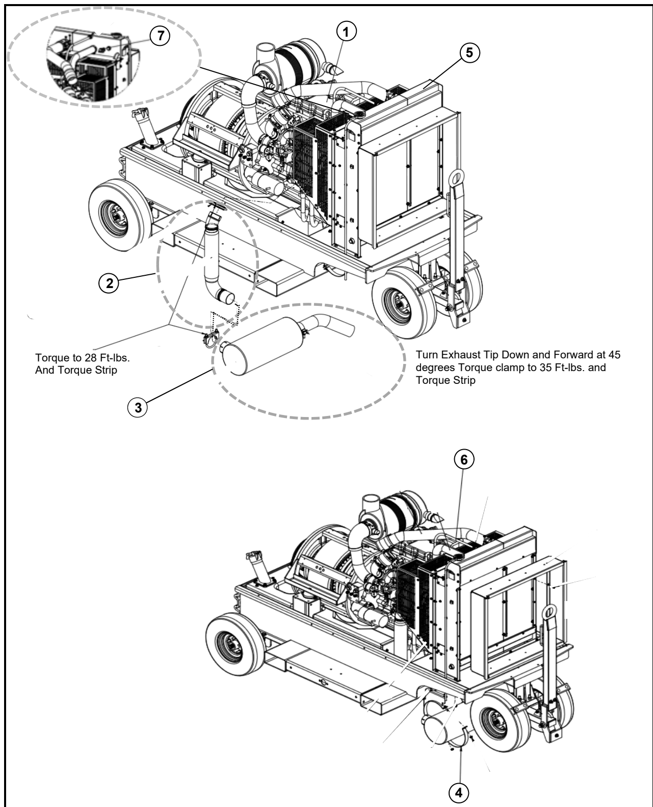
Figure 3-6. 4400-T3, Radiator/Exhaust Installation, 60/90/100 kVA (Sheet 1 of 2).
