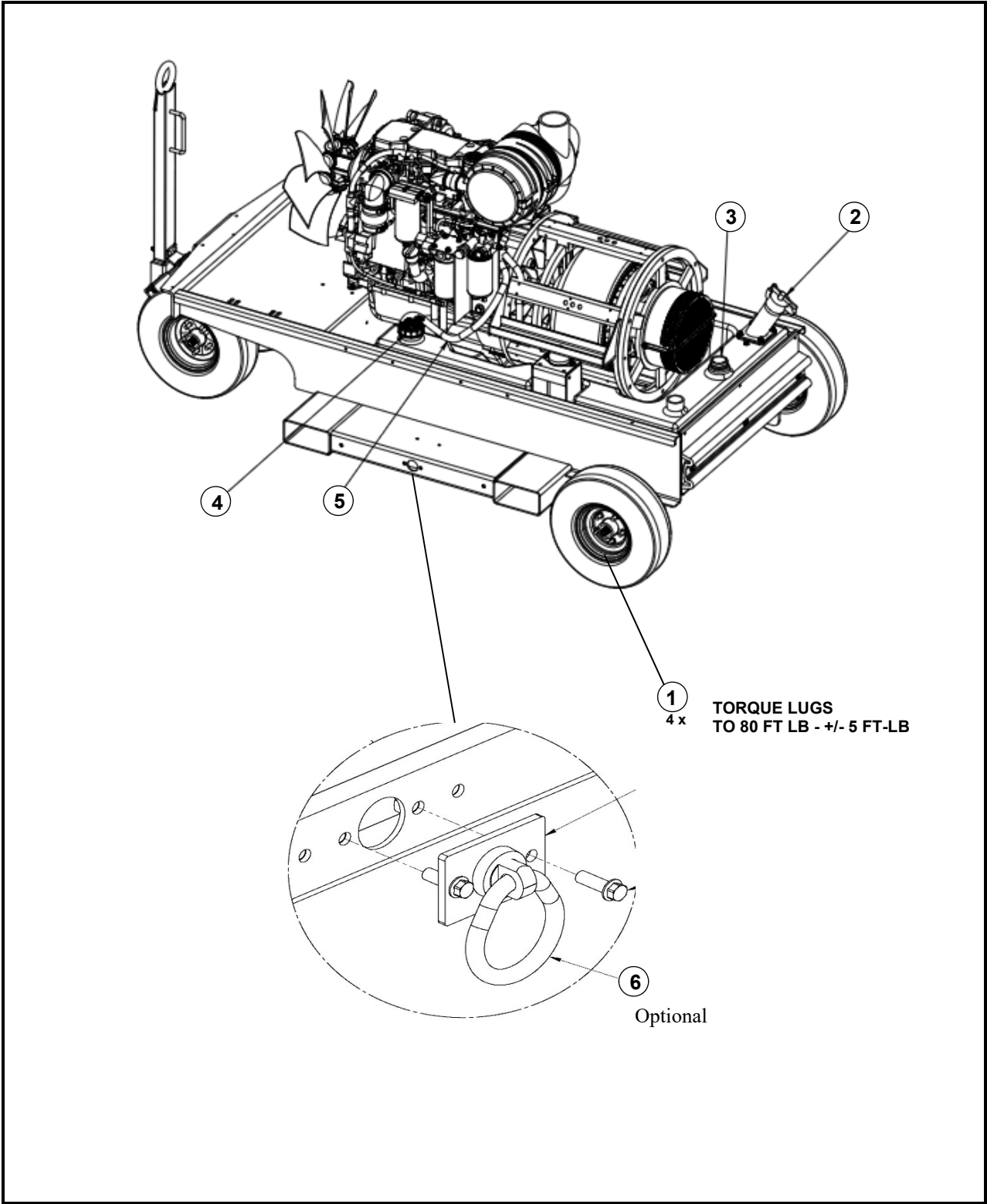
Figure 3-3. 4400-T3, Genset/Fuel Tank Installation, 60/90/100 kVA (Sheet 1 of 3).
