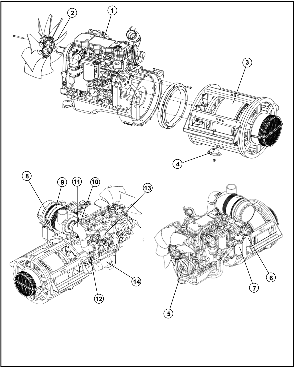
Figure 3-4. 4400-T3, Genset Assembly, 60/90/100 kVA (Sheet 1 of 2).
