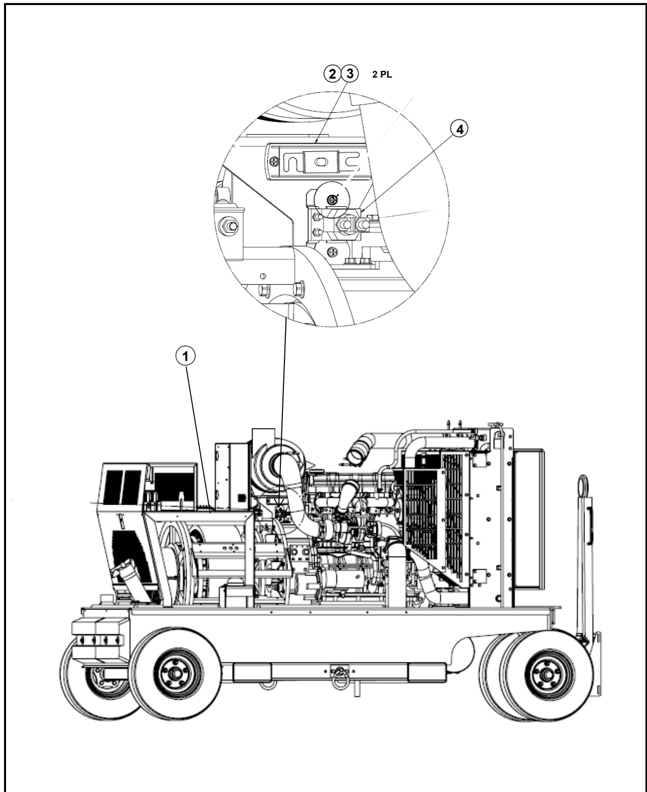
Figure 3-8. 4400-T3, Electrical System Installation, 60/90/100 kVA (Sheet 1 of 2).
