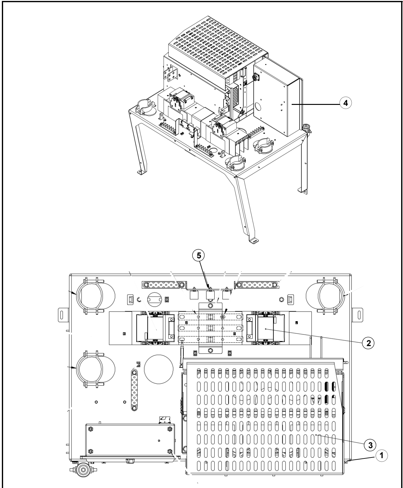
Figure 3-9. 4400-T3, Output Table Assembly, 60/90/100 kVA (Sheet 1 of 2).
