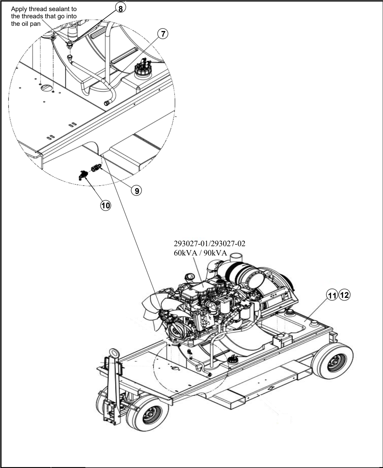
Figure 3-3. 4400-T3, Genset/Fuel Tank Installation, 60/90/100 kVA (Sheet 2 of 3).
