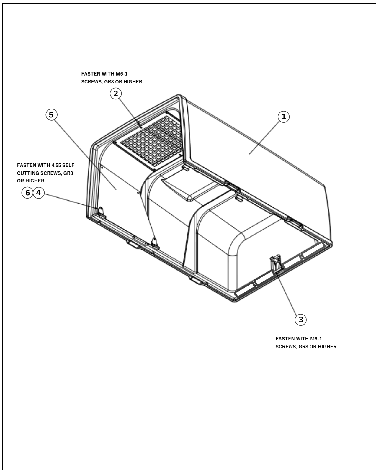
Figure 3-12. Top Canopy, Composite, Assembly 60-90 kVA (Sheet 1 of 2).
