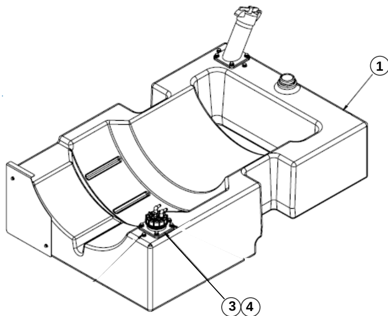
Figure 3-5. 4400-CP, Fuel Tank Composite Assembly, 60-90 kVA (Sheet 1 of 2).
