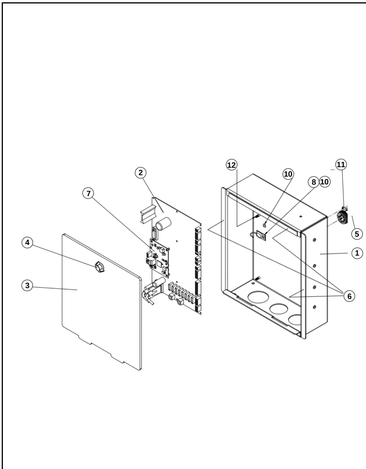
Figure 3-10. Control Module Box Assembly 60-90 kVA (Sheet 1 of 2).
