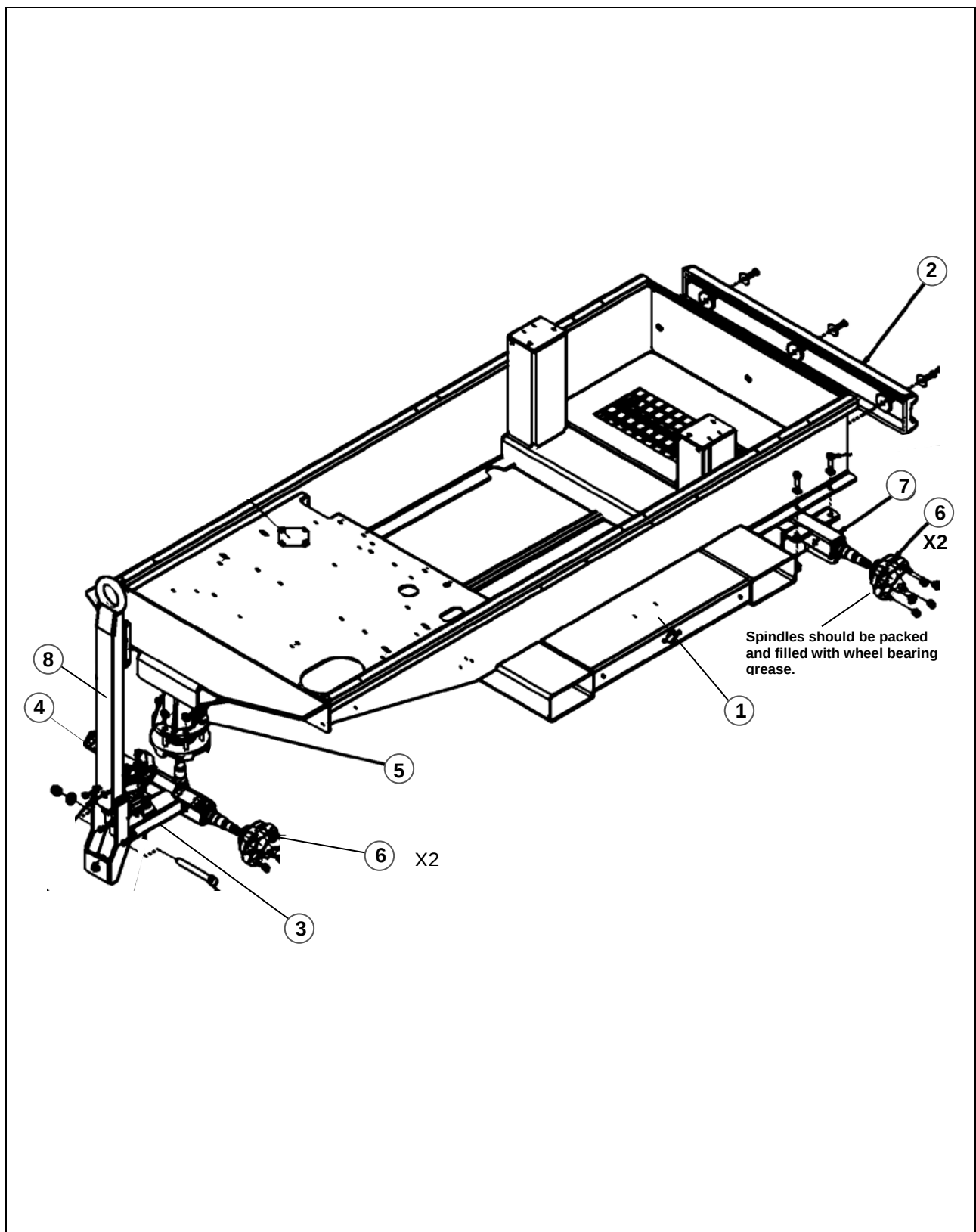
Figure 3-2. 4400-T4 Chassis/Running Gear (Sheet 1 of 2).
