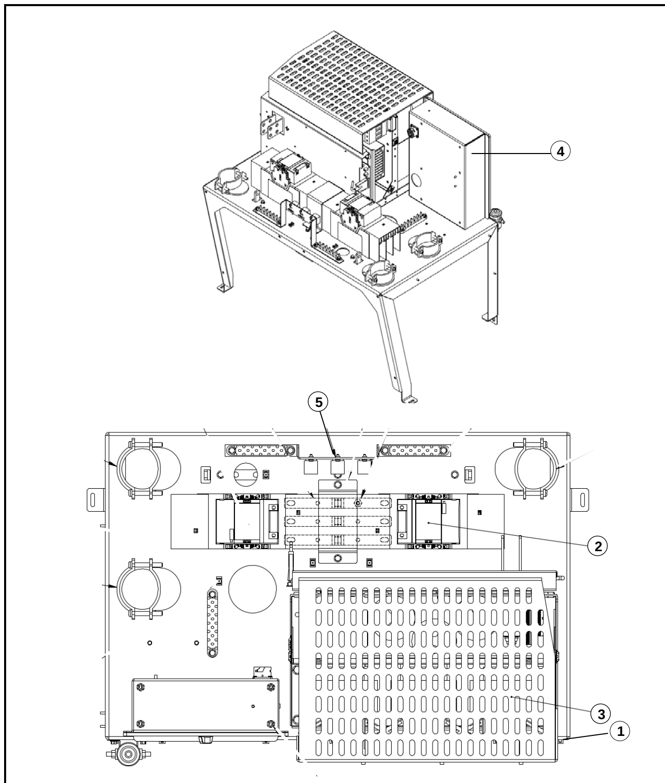
Figure 3-9. Single Output Table Assembly, W/28VDC ARU 60-90 kVA (Sheet 1 of 2).
