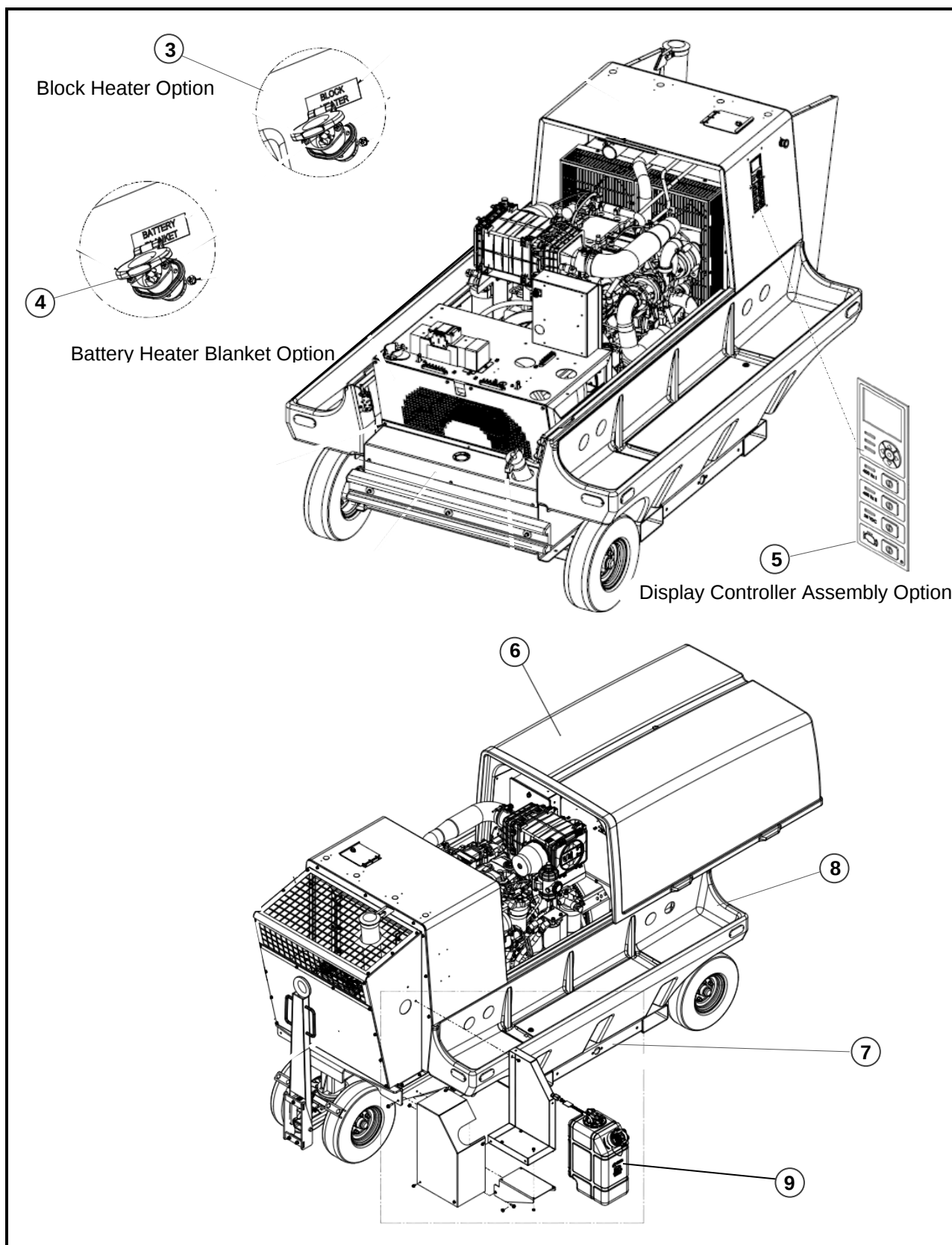
Figure 3-1. 4400-T4, 60-90 kVA, 3-Phase 115 Volt Generator Set (Sheet 2 of 3).
