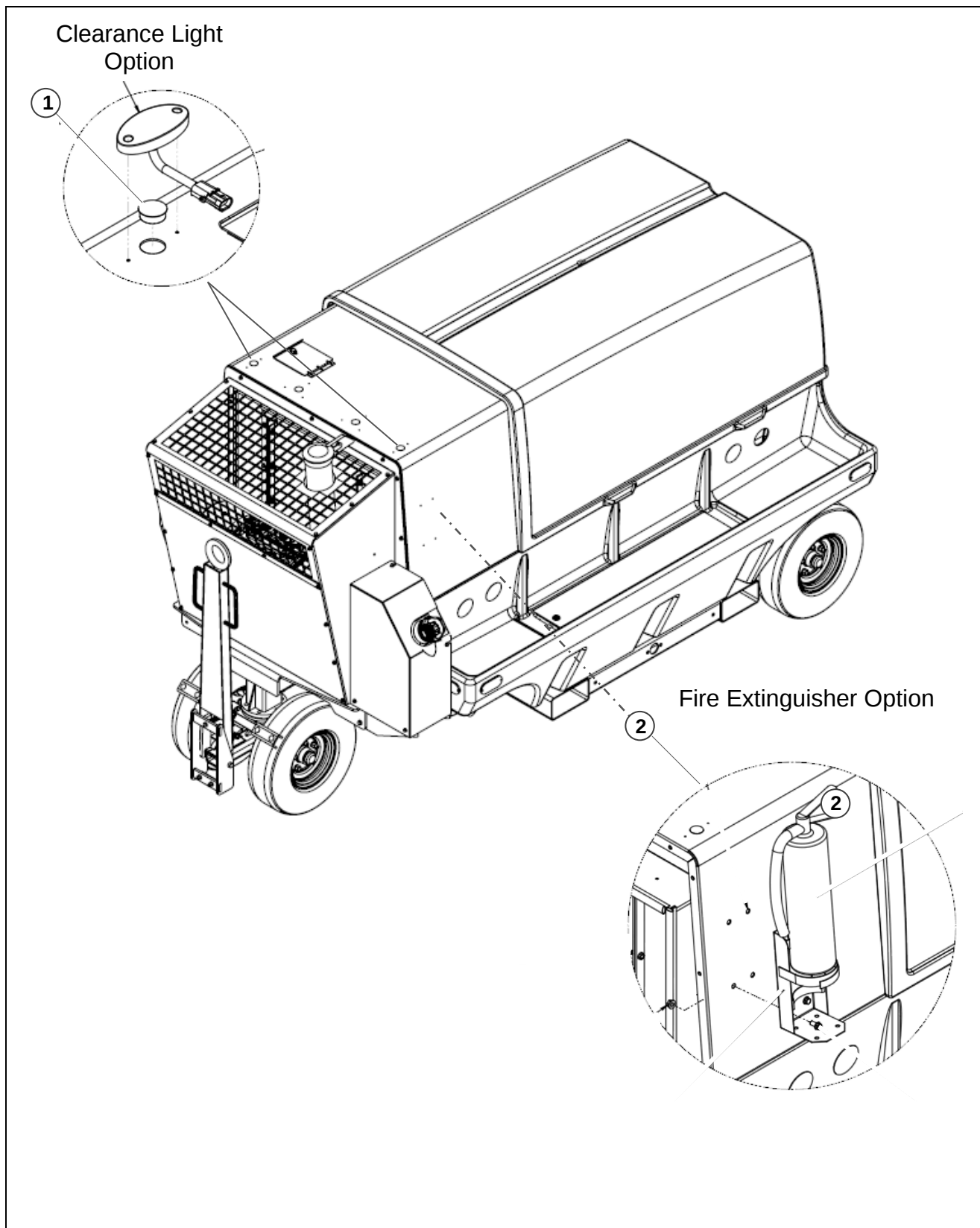
Figure 3-1. 4400-T4, 60-90 kVA, 3-Phase 115 Volt Generator Set (Sheet 1 of 3).
