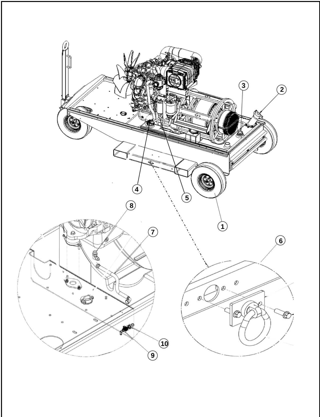
Figure 3-3. Genset/Fuel Tank Installation, 60-90 kVA (Sheet 1 of 3).
