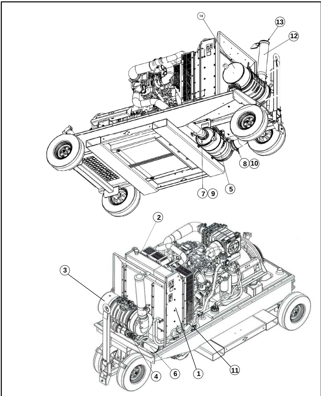
Figure 3-6. Radiator/After-Treatment Installation, 60-90 kVA (Sheet 1 of 2).
