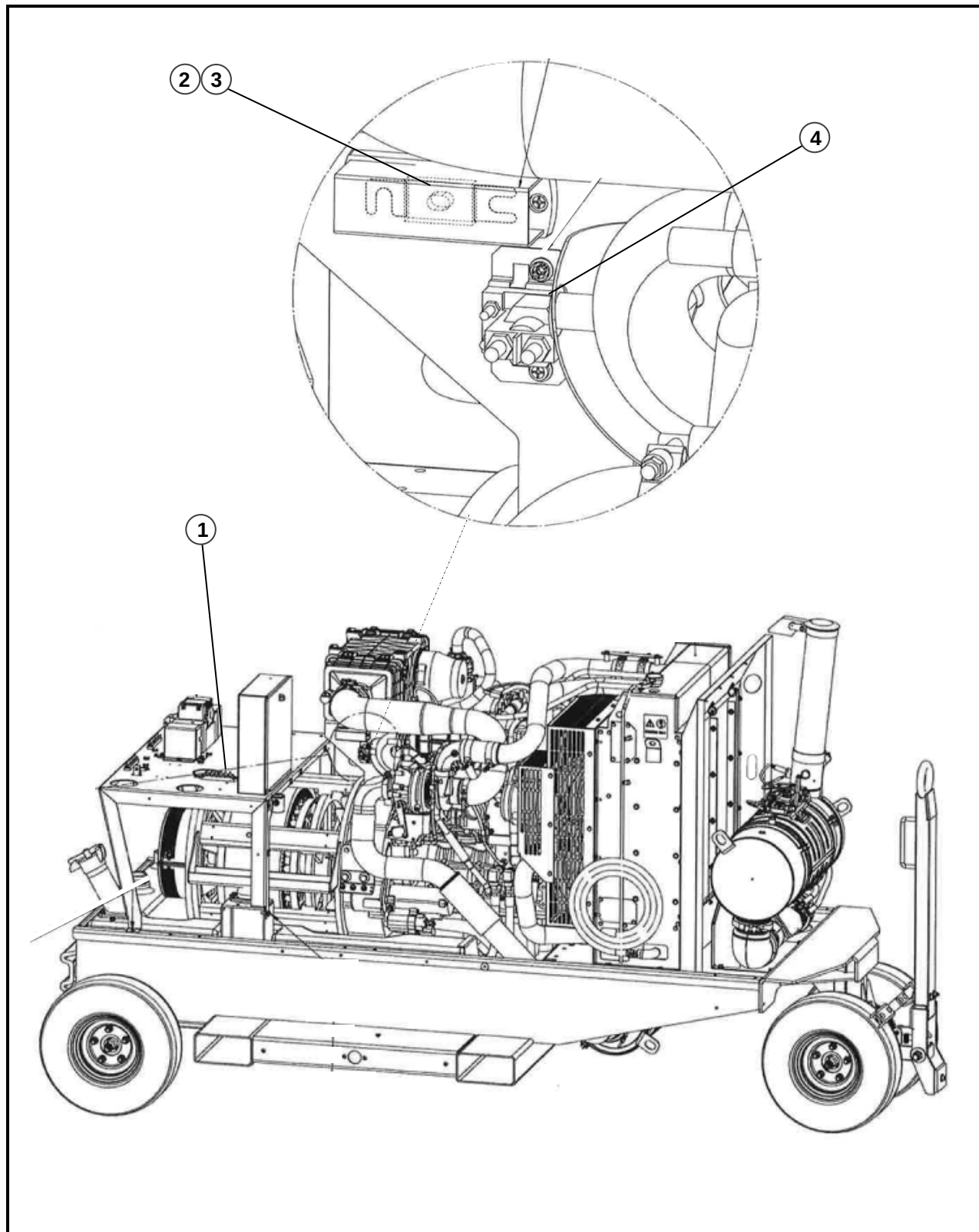
Figure 3-8. 4400-T4, Electrical System Installation, 60-90 kVA (Sheet 1 of 2).
